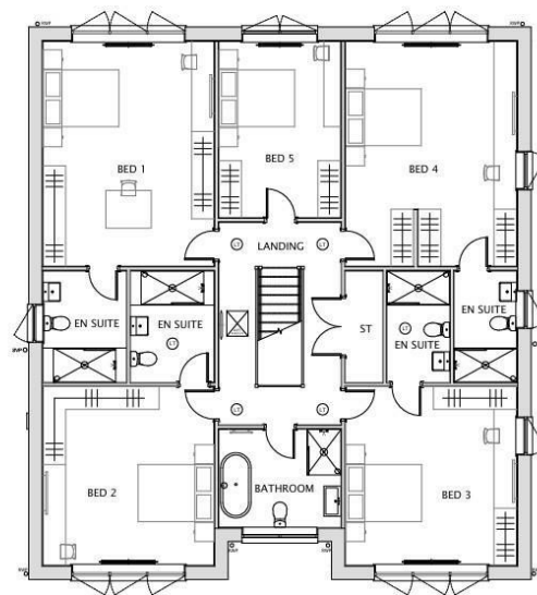
FIRST FLOOR PLAN 170 M 2 / 1830 SQ.FT
